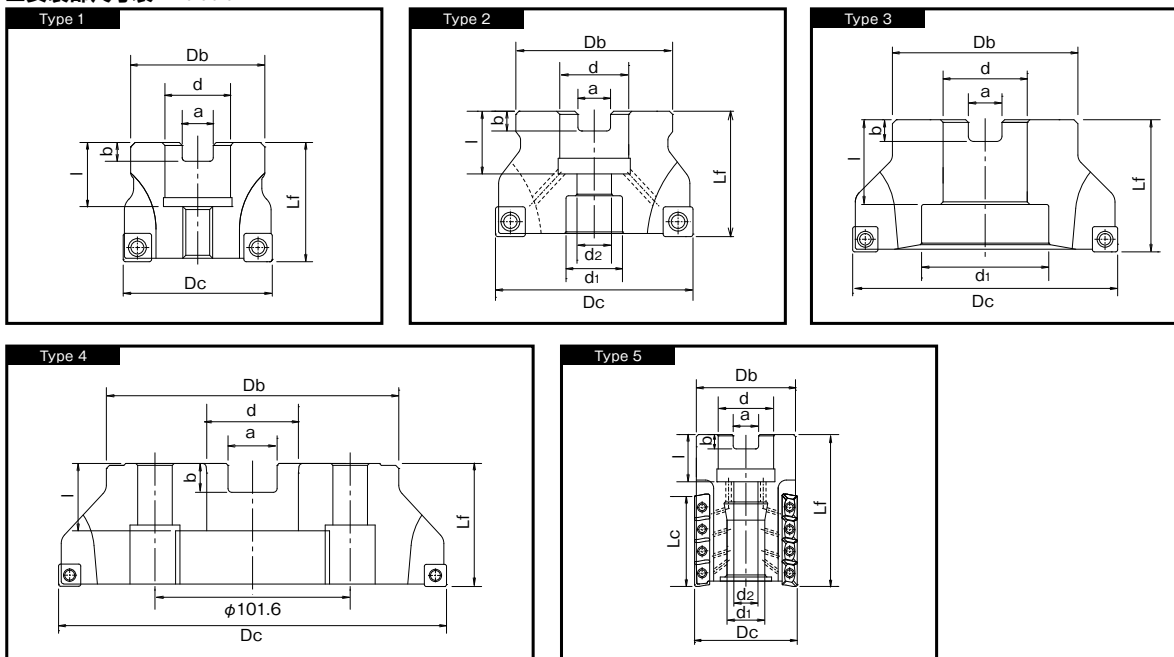
刀盘型刀具 Bore Type Cutter
