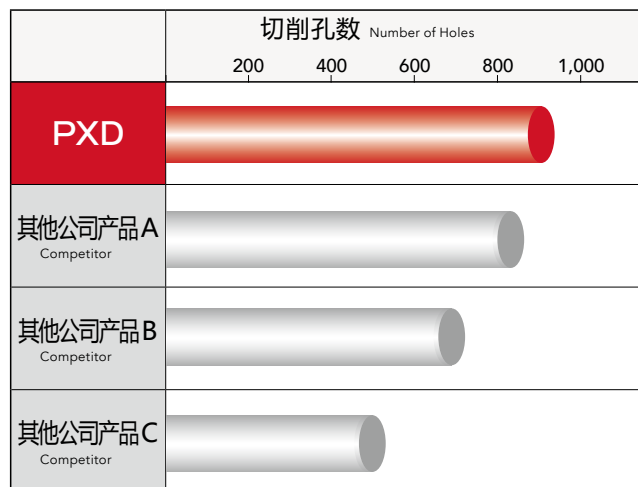
加工700孔时的磨损比较 Wear comparison after 750 holes of drilling
