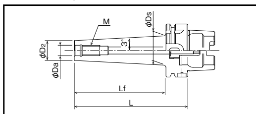
HSK 刀柄夹具 HSK Shank Holder
