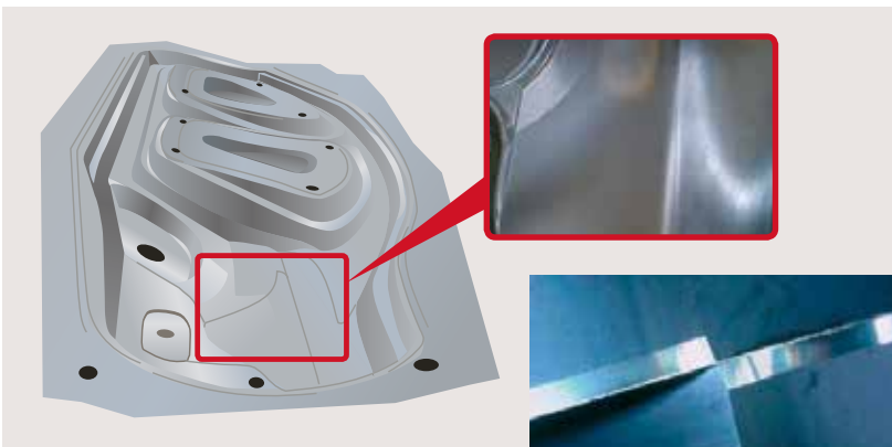
加工51小时后的刀尖状态 Cutting edge after 51 hours of milling
