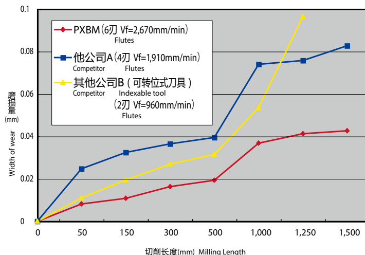
[PXB] NAK80的斜面加工(每刃进给相同时的比较) NAK80 machining at slop face (comparison in the same feed rate)
